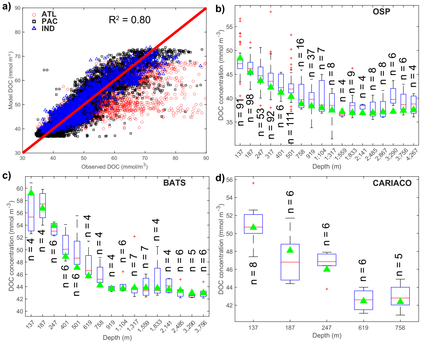
Extended Data Fig. 4 | Comparison of model DOC (DOC + DOC + + DOC - ) based on SeaWiFS CbPM NPP field to observations. a, Tracer-tracer comparison for DOC between the observations and the optimal model. Red circles show DOC observations in the Atlantic Ocean, black squares in the Pacific Ocean, blue triangles in the Indian Ocean and green stars in the Arctic Ocean. The red line shows the one-to-one line. The model captures roughly 80% of the spatial variance of the DOC data. b-d, Comparisons of model DOC to those measured
