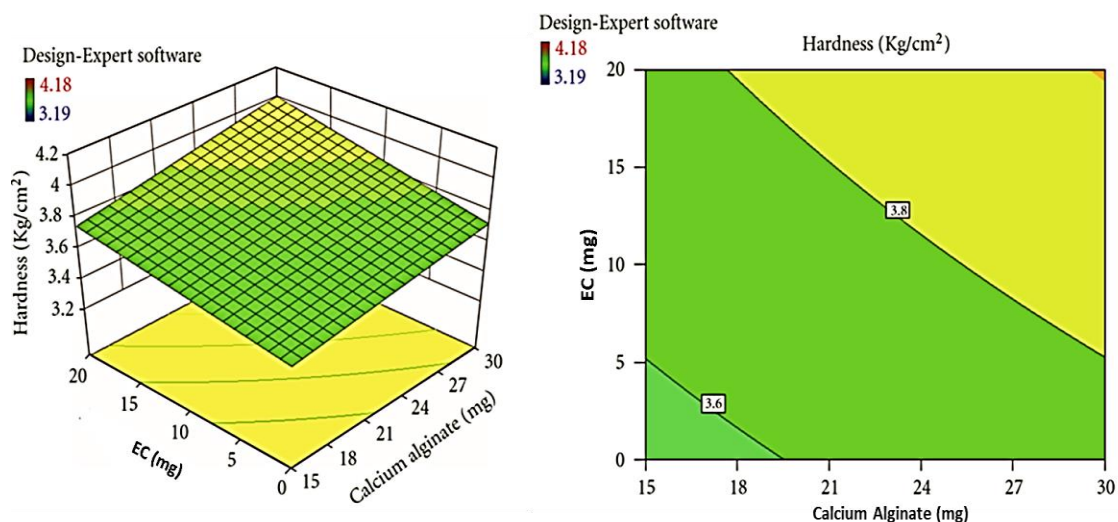
Fig. 8. The RSP [A] and CP [B] illustrate the impact of varying amounts of calcium alginate and EC on the hardness (kg/cm 2 )
