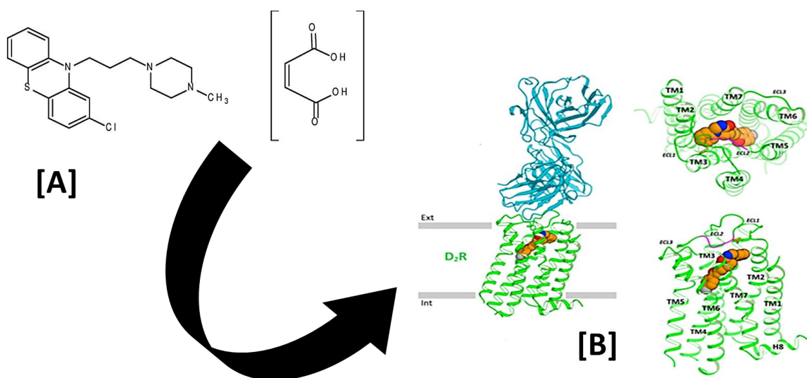
Fig. 2. The Structure of the dopamine D2 receptor in complex with the PCM drug [A]. Chemical structure of PCM and [B]. The docking of PCM
